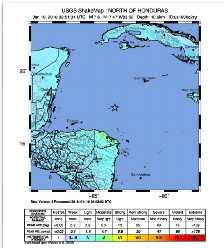
Figure 2: Earthquake shake map showing epicentre north of Honduras
